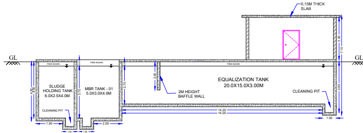
CROSS SECTION ALONG B-B
